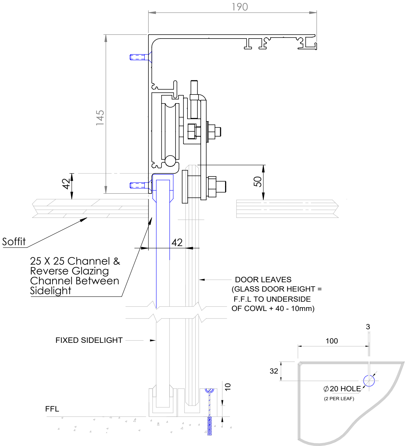
GLASS DRILLING DETAIL
