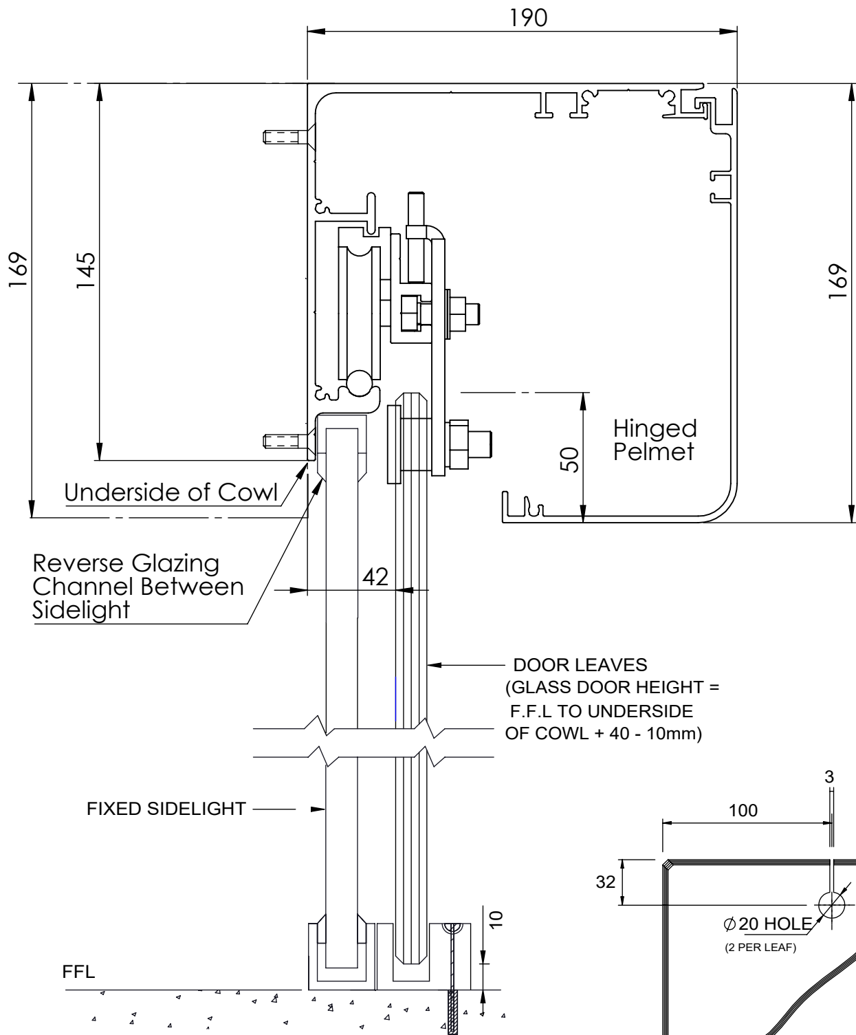
GLASS DRILLING DETAIL
