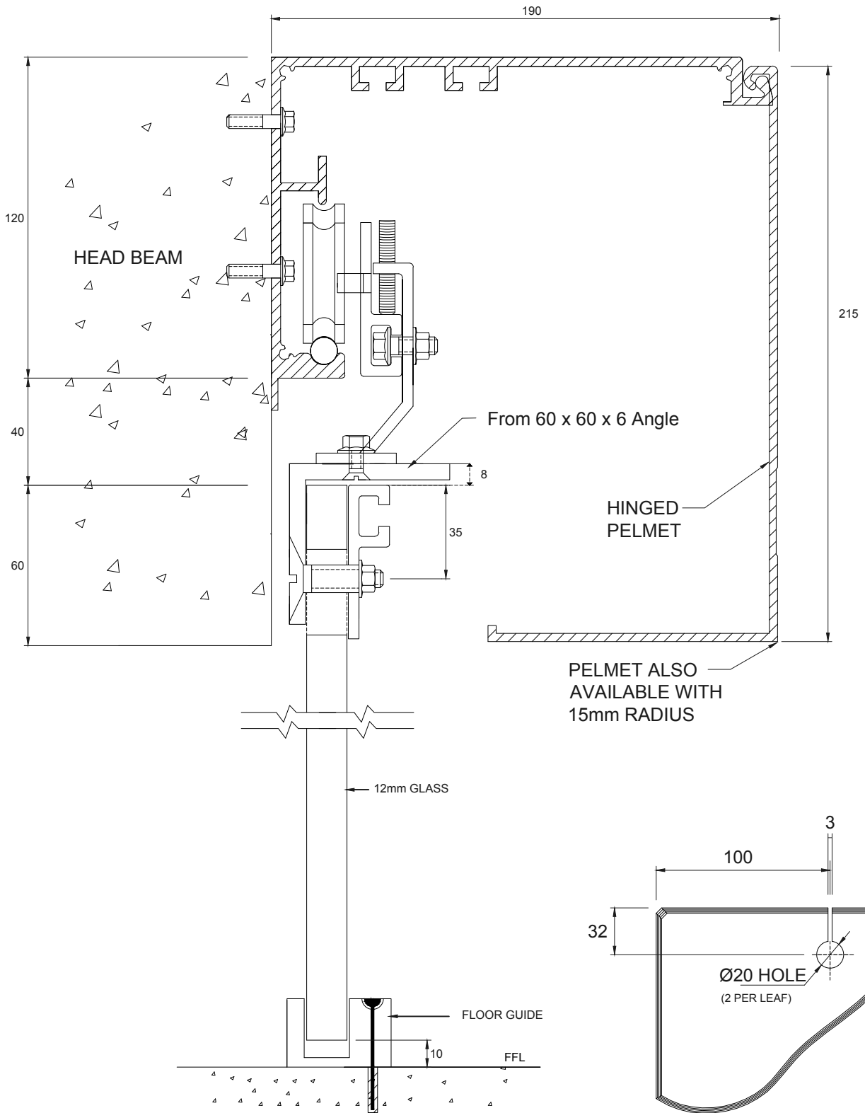
GLASS DRILLING DETAIL
