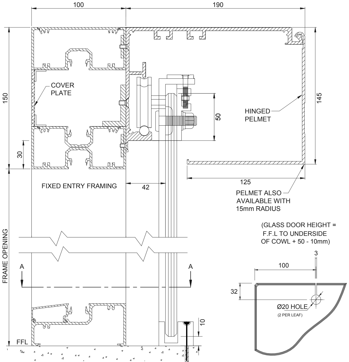
GLASS DRILLING DETAIL
