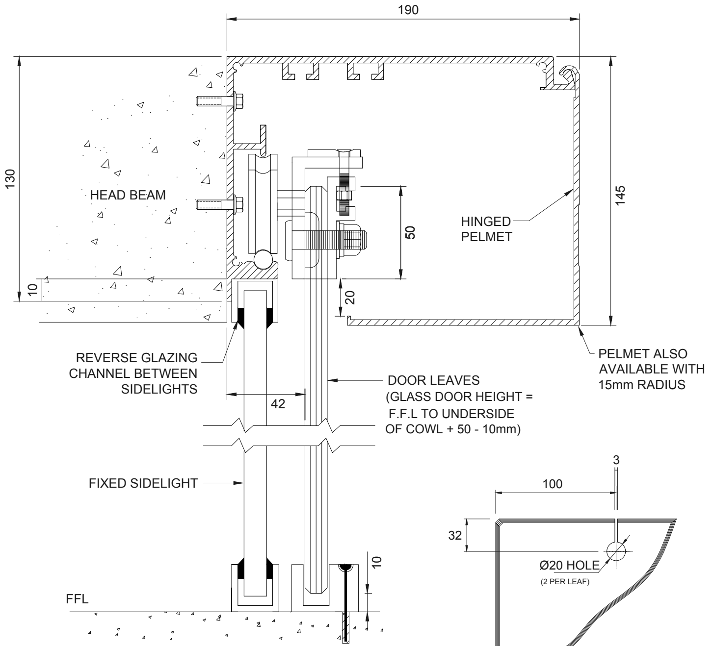
GLASS DRILLING DETAIL
